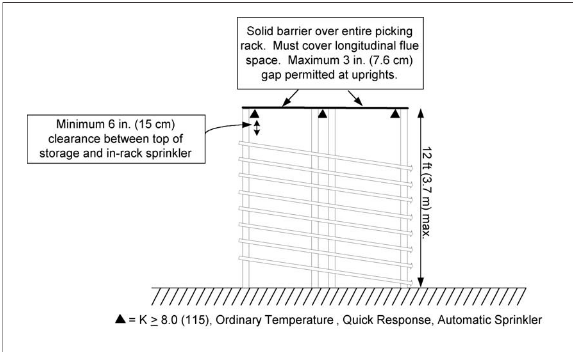
Fig. 12a. Aerosol product picking area elevation view
