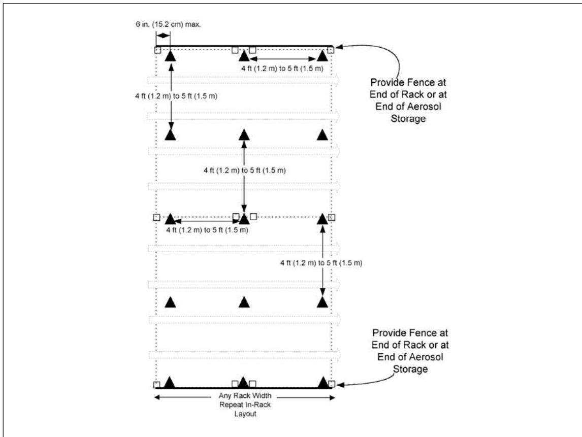
Fig. 12b. Aerosol product picking area plan view
